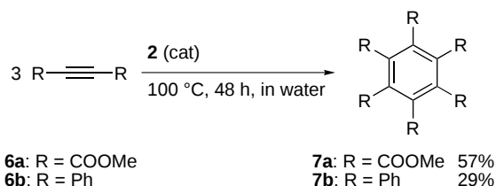
Scheme 3. Rh-catalyzed trimerization of alkynes in water.
