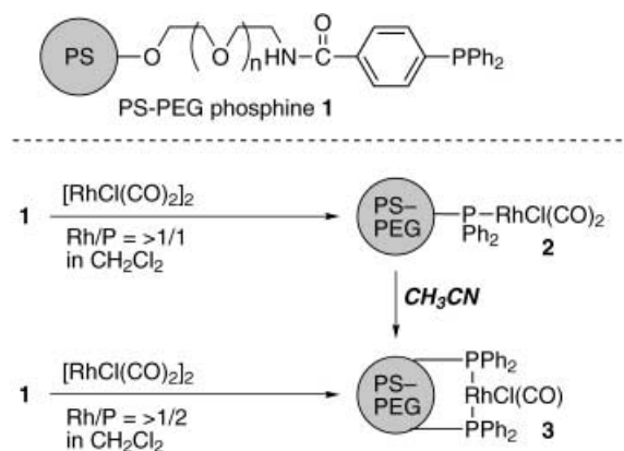
Scheme 1. Preparation of PS-PEG-supported Rh-phosphine complexes 2 and 3 .
